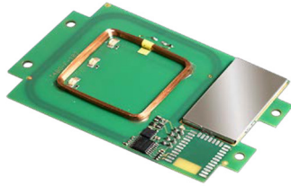
T4 MultiTech 2 LF PCB top view
